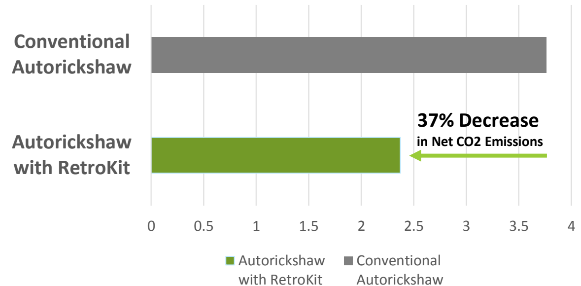
CO 2 Emissions Per Year (per vehicle) (t)
